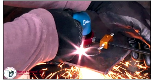
The Plasma Wiz will cut holes from 7/8" to 12" Dia. without any wheels.
