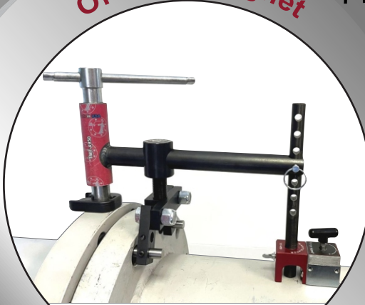
Magnetic Digital Centering Head
